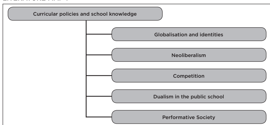
FIGURE 1 LITERATURE MAP 1
