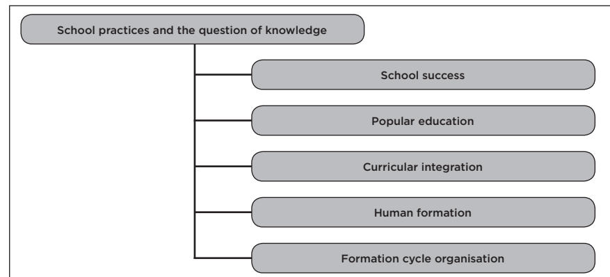
FIGURE 2 LITERATURE MAP 2
